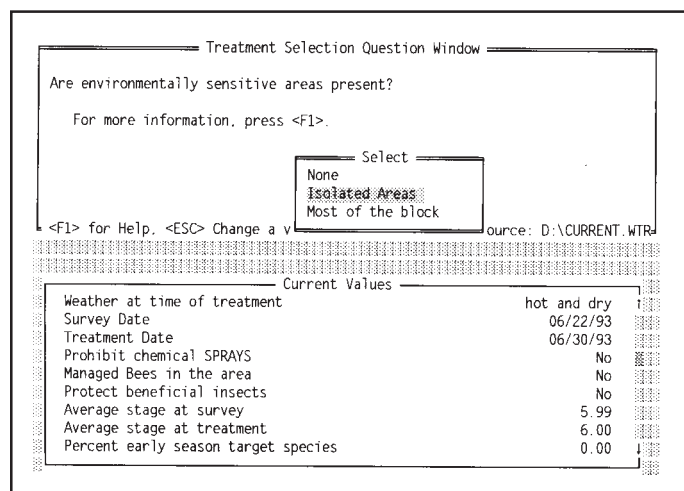
Figure VI.2-5—Typical multiple-choice data entry in Consult .
