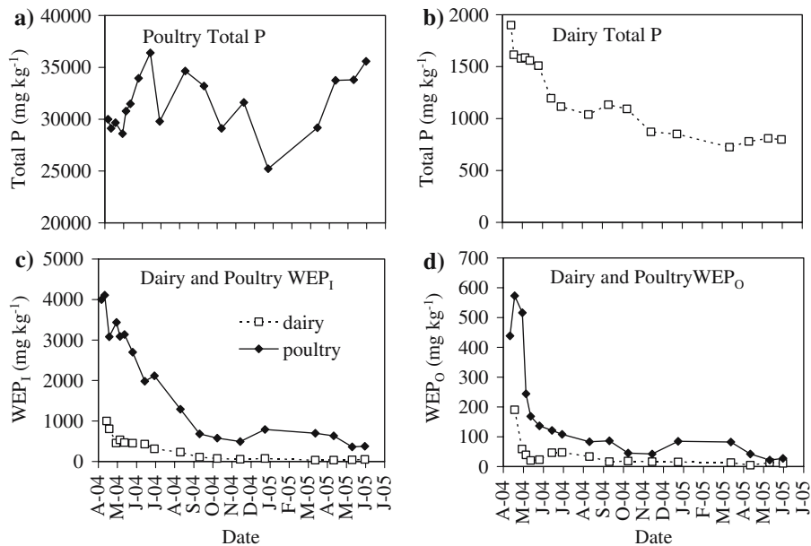
Fig. 5 Changes in the concentrations ( \text{mg kg}^{-1} ) of (a) poultry manure total P, (b) dairy manure total P, (c) dairy and poultry manure \text{WEPI} , and (d) manure \text{WEP}_O for Pennsylvania bare and grassed plots
