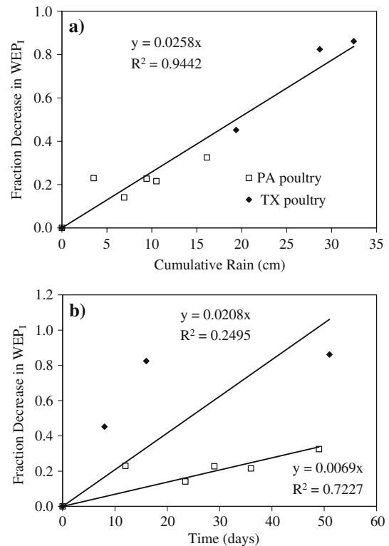
Fig. 6 The relationship between the fraction decrease in manure WEP I during the experiments and (a) the cumulative precipitation (cm) or (b) time (days) for both Texas grassed plots and Pennsylvania grassed and bare plots
