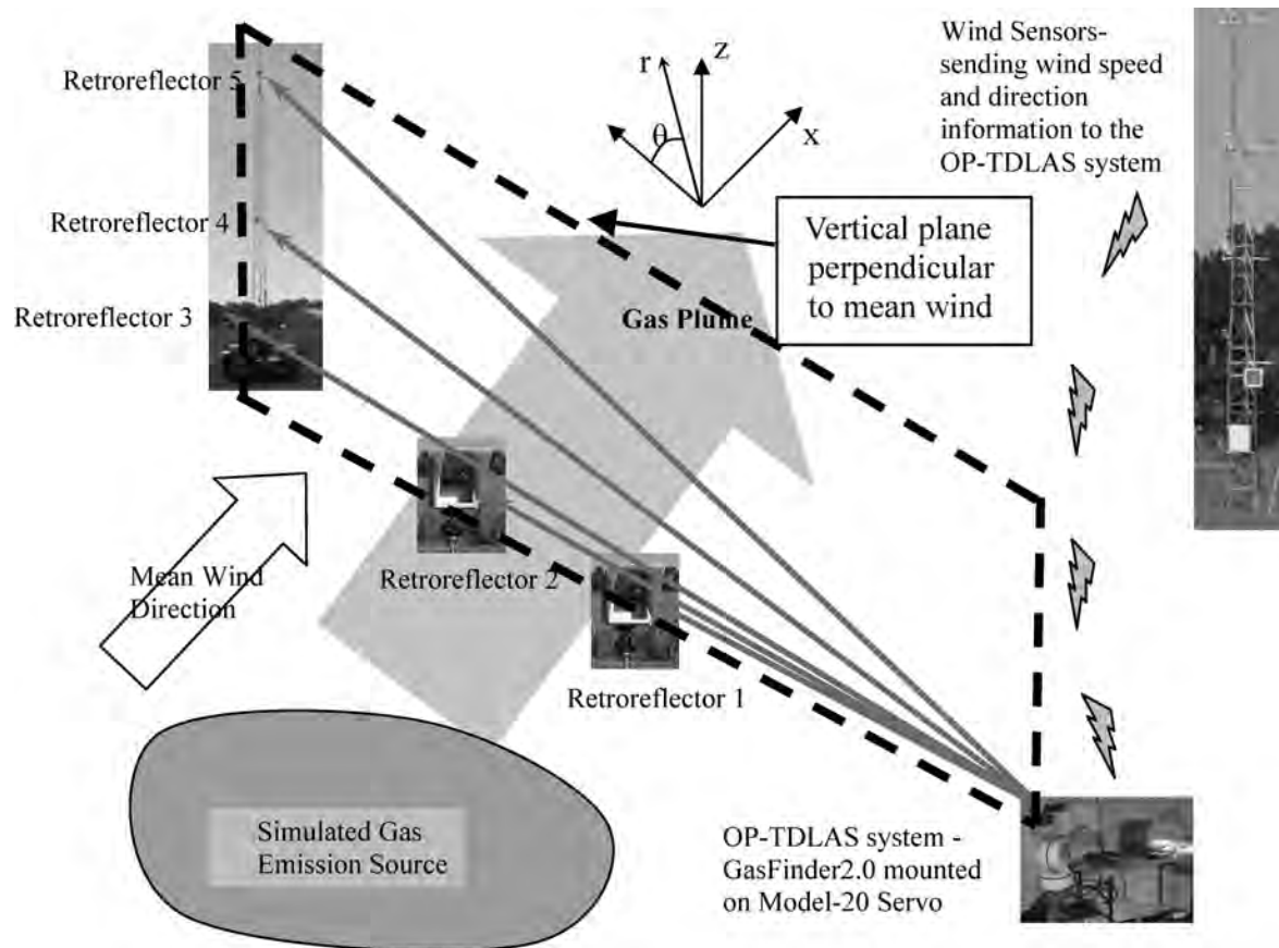
Fig. 1. Simulated field configuration and OP-TDLAS beam geometry.
