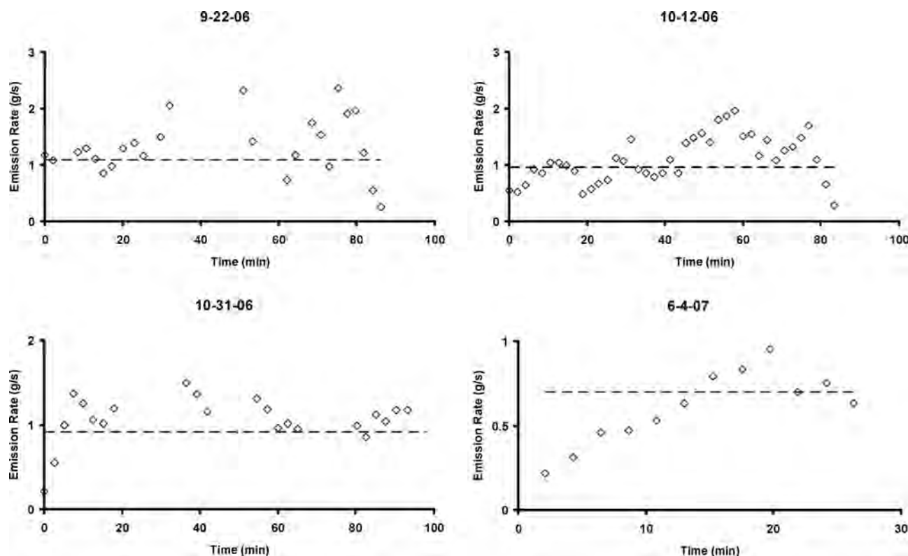
Fig. 5. VRPM estimates and average CH 4 release rates for the 4 validation studies (◇ VRPM estimates, — Average release rate).
