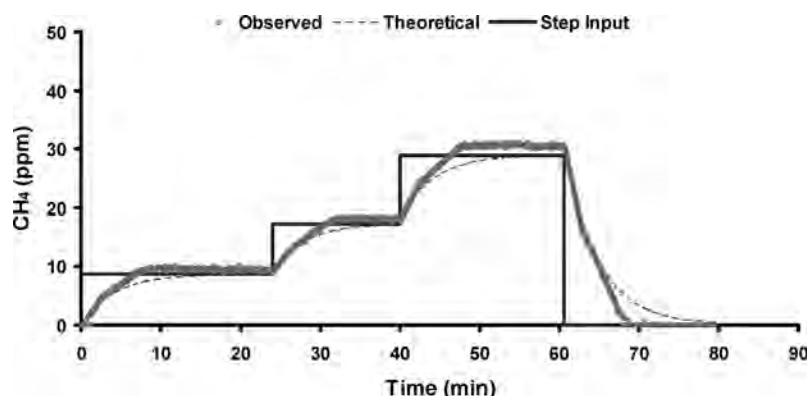
Fig. 3. Comparison of theoretical and observed \text{CH}_4 concentration in the PVC pipe.
