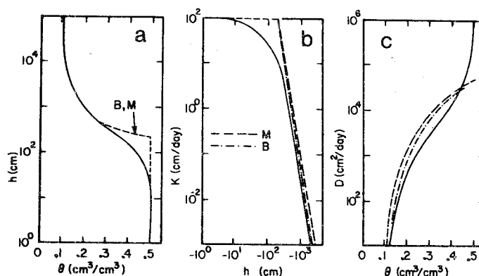
Fig. 4—Comparison of the proposed soil hydraulic functions (solid lines) with curves obtained by applying either the Mualem theory ( M ; dashed lines) or the Burdine theory ( B ; dashed-dotted lines) to the Brooks and Corey model of the soil-water retention curve.
