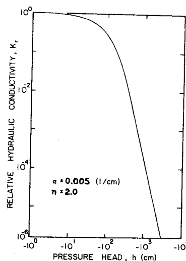
Fig. 2—Plot of the relative hydraulic conductivity vs. pressure head as predicted from knowledge of the soil-water retention curve shown in Fig. 1.
