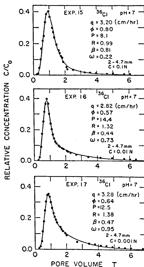
Fig. 6. Measured 36 Cl breakthrough curves through column 3. The dots represent experimental data points, and the lines are calculated with model II.
