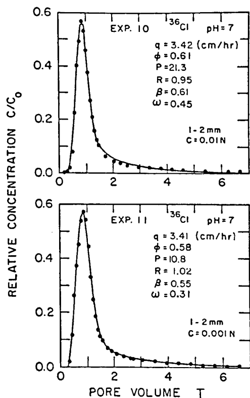
Fig. 8. Measured ^{36}\text{Cl} breakthrough curves through column 2. The dots represent experimental data points, and the lines are calculated with model II.
