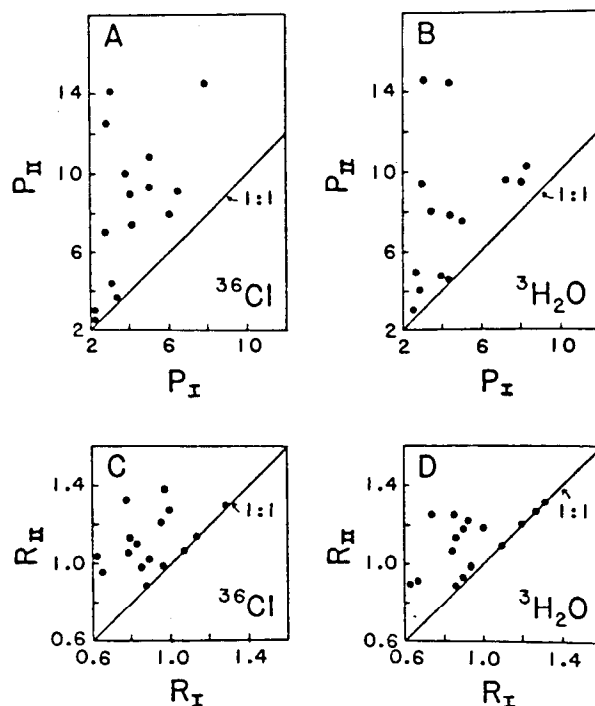
Fig. 9. A comparison of the Peclet number P and the retardation factor R estimated with model I and model II from ^3\text{H}_2\text{O} and ^{36}\text{Cl} breakthrough curves. (a) Peclet number with model I ( P_I ) and with model II ( P_{II} ) for ^{36}\text{Cl} . (b) Peclet number P for ^3\text{H}_2\text{O} . Retardation factors R for ^{36}\text{Cl} . (d) Retardation factors R for ^3\text{H}_2\text{O} .
