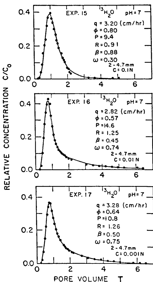
Fig. 5. Measured 3 H 2 O breakthrough curves through column 3. The dots represent experimental data points, and the lines are calculated with model II.
