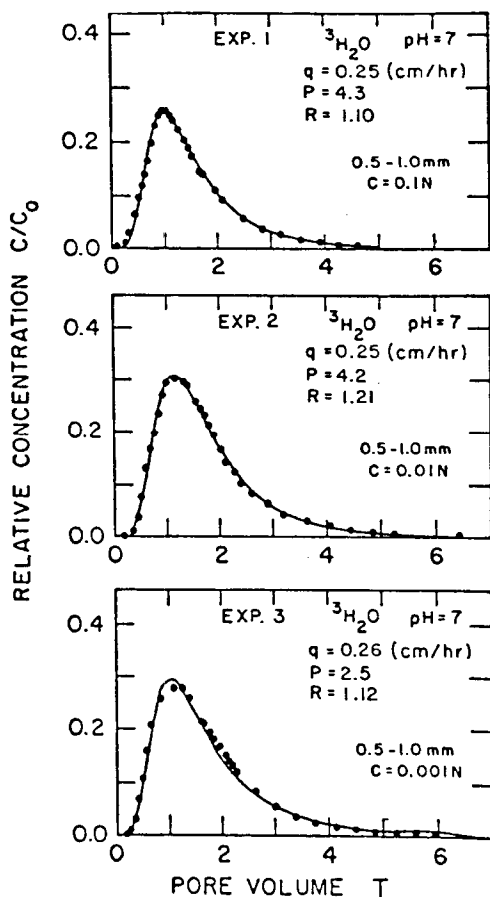
Fig. 1. Measured ^3\text{H}_2\text{O} breakthrough curves through column 1. The dots represent experimental data points, and the lines are calculated with model I.
