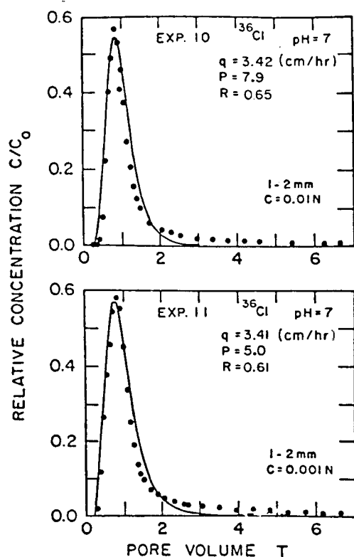
Fig. 7. Measured ^{36}\text{Cl} breakthrough curves through column 2. The dots represent experimental data points, and the lines are calculated with model I.
