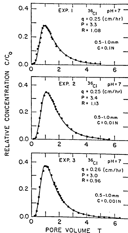
Fig. 2. Measured ^{36}\text{Cl} breakthrough curves through column 1. The dots represent experimental data points, and the lines are calculated with model I.
