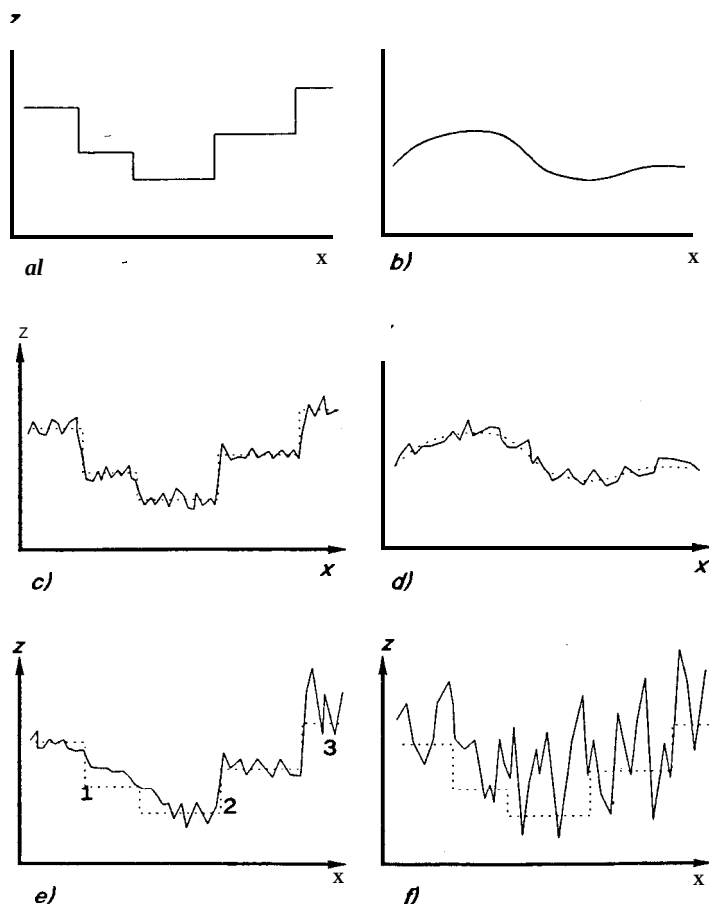
Fig. 1. Hypothetical models of various forms of spatial variation that can occur in soil. (a) Idealized homogenous variation within map units having sharp boundaries that are often used to approximate some of the following real kinds of variation. (b) Continuous smooth variation, typical of some landforms. (c) Within-unit variation smaller than between unit variation as can occur when soil variation is dominated by differences in homogeneous geological units. (d) Continuous smooth variation with local noise that is common for many hydrological properties such as groundwater levels. (e) Non-stationary variation including a trend (1), abrupt change (2) and larger than average within-unit variation (3) that occurs with many soil attributes. (f) Variation where short range effects such as periglacial features or local levels of soil pollutants can swamp all other signals.
