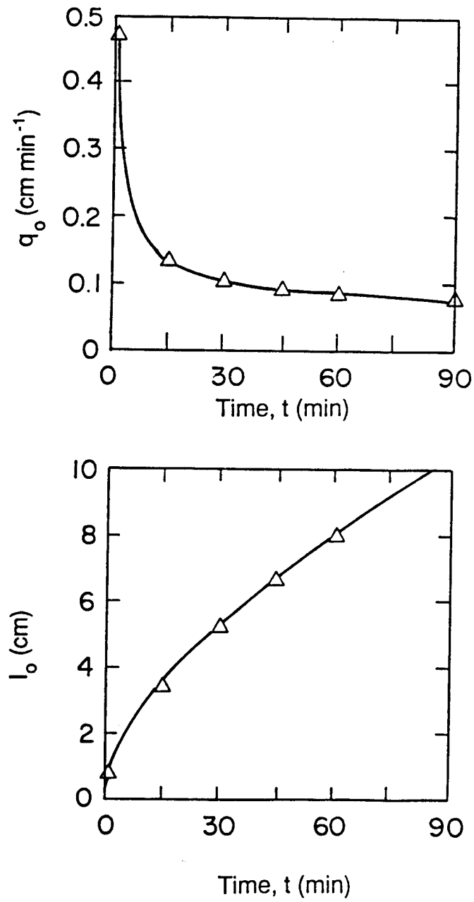
Fig. 7.3. Instantaneous, q_o , and cumulative, I_o , infiltration rates simulated with the SWMS_2D (solid lines) and UNSAT2 (triangles) codes for example 1.
