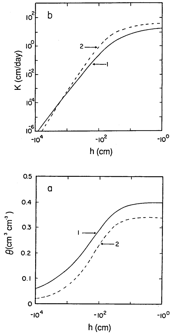
Fig. 7.5. Unsaturated hydraulic properties of the first and second soil layers for example 2.
