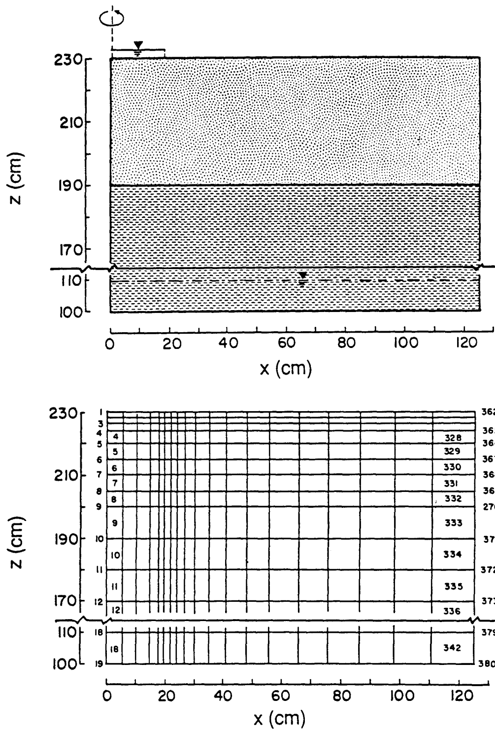
Fig. 7.14. Flow system and finite element mesh for example 4.
