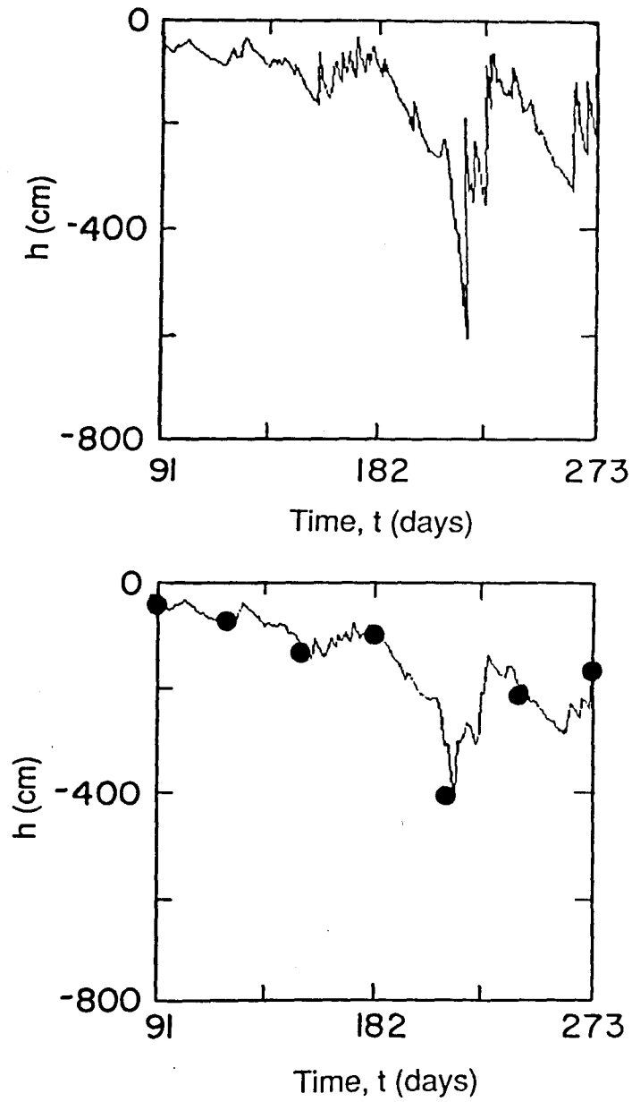
Fig. 7.8. Pressure head at the soil surface and mean pressure head of the root zone for example 2 as simulated with SWMS_2D (solid lines) and SWATRE (solid circles).
