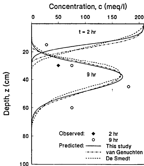
FIG. 4. Observed and calculated chloride concentration profiles during ponded infiltration in a Panoche clay loam (Warrick et al. 1971).
