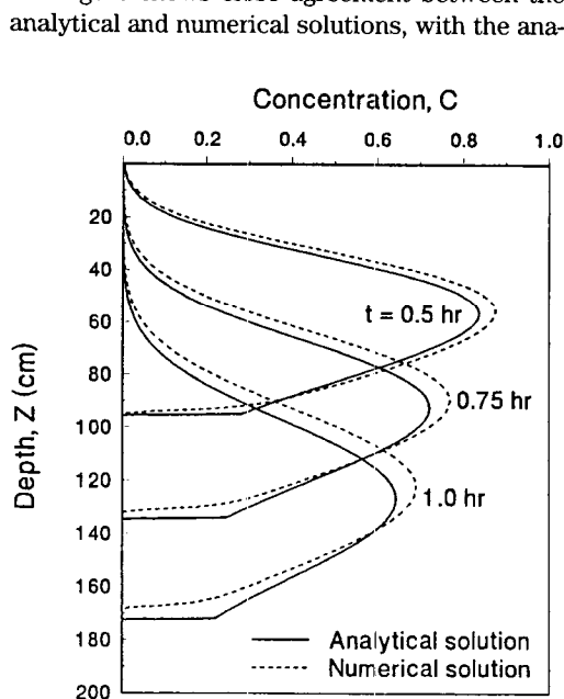
FIG. 2. Comparison of the proposed analytical solution with numerical results for solute transport in a coarse-textured soil.
