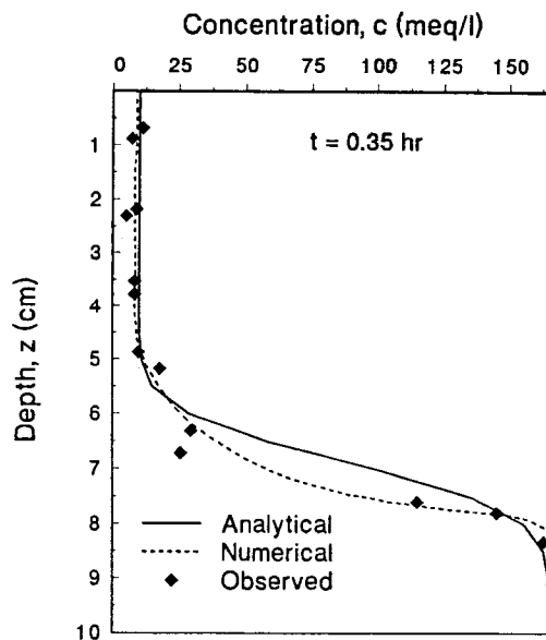
FIG. 3. Observed (diamonds) and calculated chloride concentration distributions during ponded infiltration. The solid line denotes the proposed analytical solution, whereas the dashed line represents the numerical solution of Bresler and Laufer (1974).
