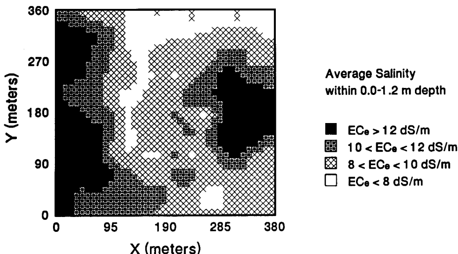
Fig. 4. Map of average rootzone (0–1.2 m) soil salinity ( EC_e basis) in a tile-drained field (silty loam soil) located in the Coachella Valley of California.
