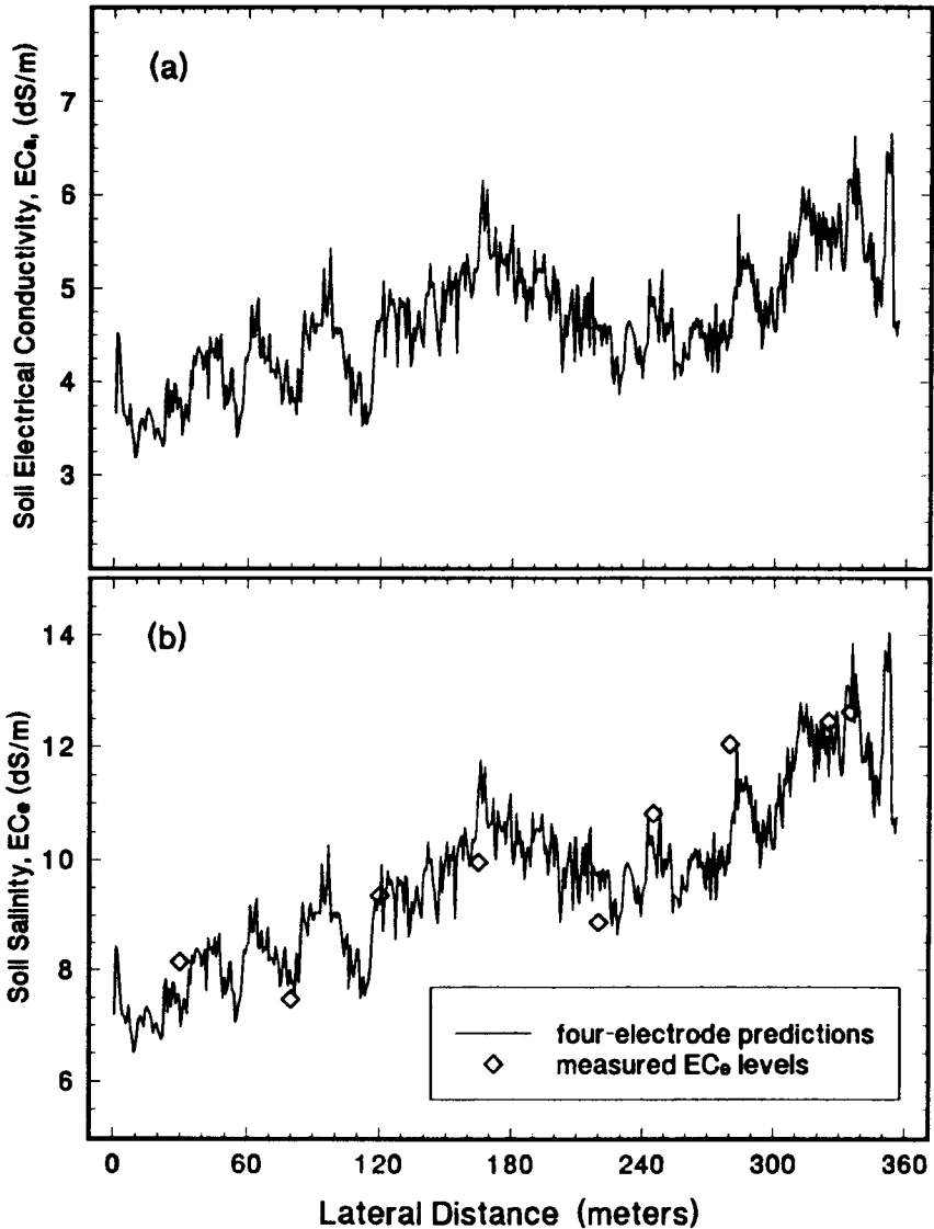
Fig. 2. Relation between (a) bulk soil electrical conductivity ( EC_a ) and (b) soil salinity ( EC_e ) and distance along a transect across a furrow-irrigated, sugar beet field (Glenbar silty clay loam soil) located in the Imperial Valley of California.
