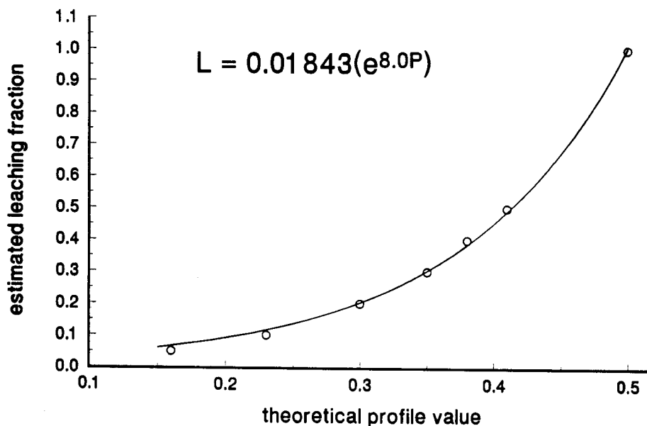
Fig. 8. Relationship between the salinity profile value and leaching fraction.
