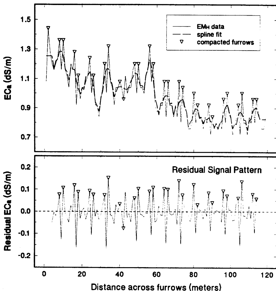
Fig. 9. Cyclic pattern of soil electrical conductivity across a succession of furrows, some trafficked by a tractor and some not.
