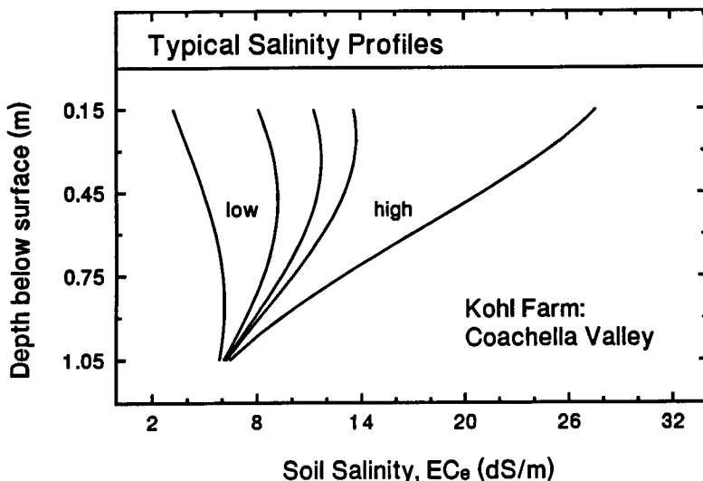
Fig. 6. Relation between salinity distribution and mean level of salinity in a tile-drained field (silty loam soil) located in the Coachella Valley of California.
