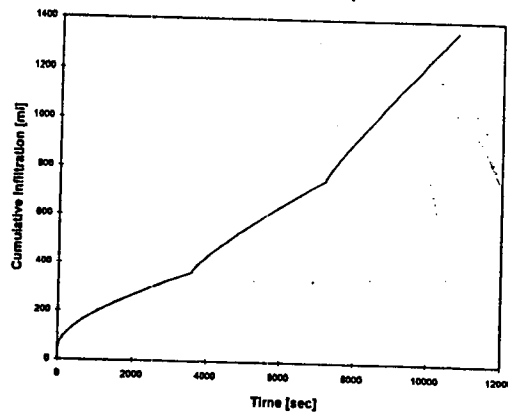
Fig. 1. Cumulative infiltration versus time for a hypothetical disc permeameter infiltration experiment with three consecutive supply pressure heads: h_0(t=0) = -20 cm, h_0(3600\text{ s}) = -10 cm, and h_0(7200\text{ s}) = -3 cm.
