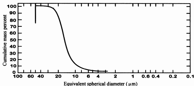
Fig. 6.1 Particle size distribution of glass spheres obtained using the Sedigraph 5000-D [Reprinted by permission of John Wiley & Sons, Inc. from Bunville, 1984. H.G. Barth (ed.) Modern methods of particle size analysis]
