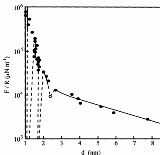
Fig. 6.12 Forces between two mica surfaces in 7 mmol L -1 NaCl electrolyte. F is the total force scaled by the radius ( R ) of the curved surfaces. At distance > 1.5 nm, the forces are described by double layer theory. Hydration forces are observed at distances < 1.5 nm [Reprinted with permission from Ducker and Pashley, 1992. Langmuir 8:109-112. Copyright American Chemical Society].
