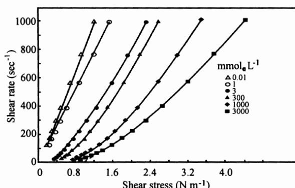
Fig. 6.18 Shear rate versus shear stress for Na-kaolinite. The open symbols represent dispersed systems and ideal plastic flow. The closed symbols represent coagulated systems and Bingham flow [Adapted from Yong et al., 1979]
