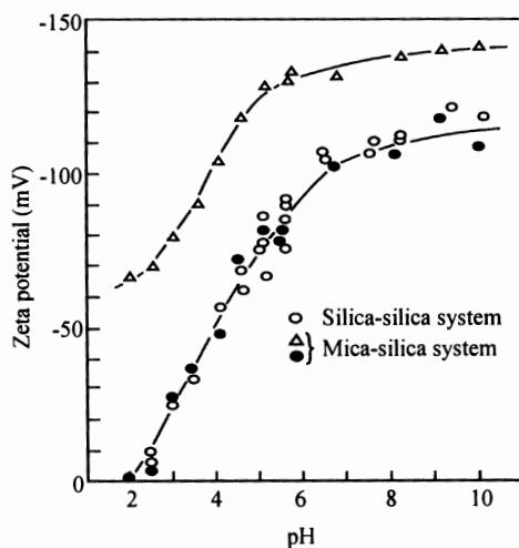
Fig. 6.5 Zeta potentials as a function of solution pH for muscovite mica basal plane-and silica plate-aqueous solution interfaces obtained using electroosmosis [Reprinted by permission of Academic Press, Inc. from Nishimura et al., 1992. J. Colloid Interf. Sci. 152:359-367]
