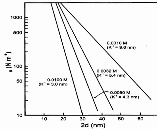
Fig. 6.11 Repulsive force between two plates for different concentrations of a 1:1 electrolyte where K is the inverse double layer distance [Reprinted by permission of Marcel Dekker, Inc. from Hiemenz, 1977. Principles of colloid and surface chemistry]
