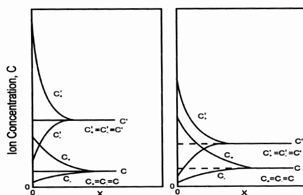
Fig 6.8 Distribution of ions in the electric double layer at two electrolyte concentrations ( c' > c ). Left: constant potential surface. Right: constant surface charge [Adapted from van Olphen, 1977. An introduction to clay colloid chemistry. Copyright John Wiley & Sons, New York with permission]
