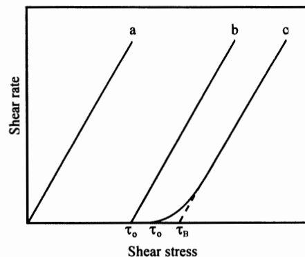
Fig. 6.17 Shear rate versus stress relationships. Curve a represents Newtonian flow, curve b represents ideal plastic flow, and curve c represents Bingham flow [Adapted from van Olphen, 1977]
