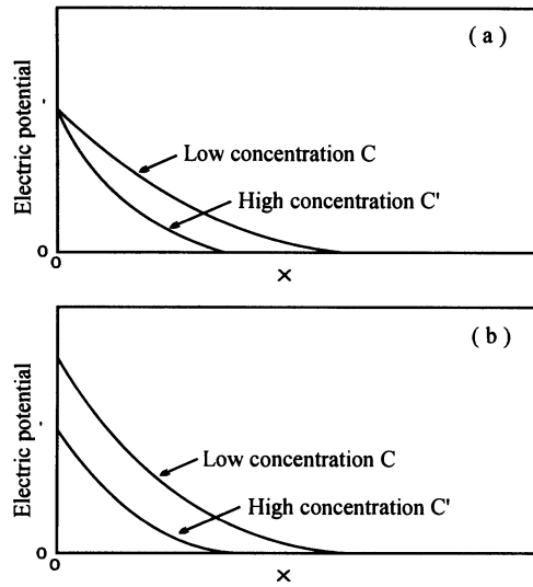
Fig. 6.9 Electrical potential distribution in the double layer at two electrolyte concentrations. Top: constant potential surface. Bottom: constant surface charge [Adapted from van Olphen, 1977. An introduction to clay colloid chemistry. Copyright John Wiley and Sons, New York with permission]
