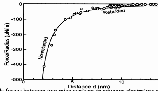
Fig. 6.10 van der Waals forces between two mica surfaces in aqueous electrolyte solutions. The measured Hamaker constant is A = 2.2 \times 10^{-20} J. Retarded van der Waals forces are observed above 5 nm [Reprinted from Israelachvili, 1992. Intermolecular and surfaces forces. Academic Press Ltd, London, UK with permission].
