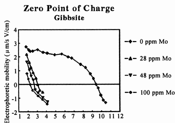
Fig. 6.3 Shifts in p.z.c. and charge reversal of gibbsite in the presence of molybdate [From Goldberg et al., 1996]
