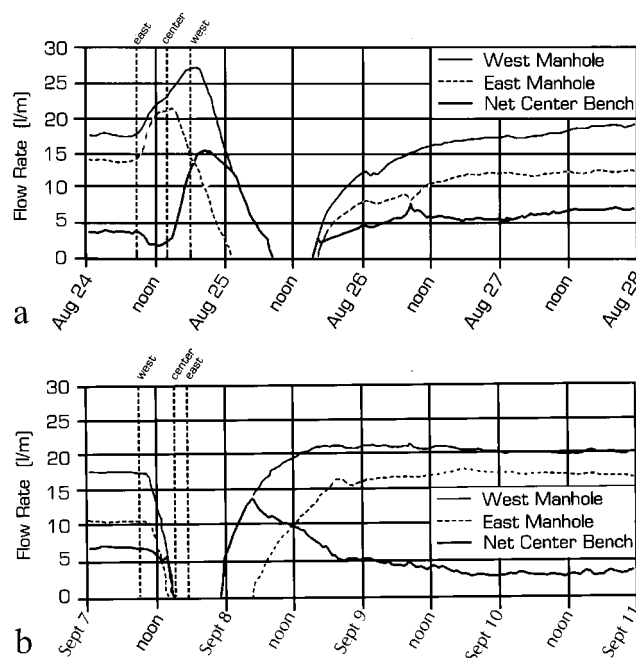
Figure 10. Typical tile flow behavior at the field site following (a) an east-center-west and (b) a west-center-east irrigation sequence. Vertical dashed lines represent irrigation starting times for the respective benches. Positive values indicate westerly flow. Occasional easterly flow are shown as zero flow.
