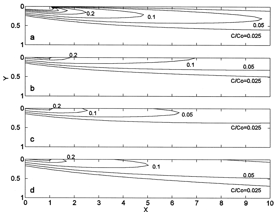
Fig. 2. Steady-state contours of the dimensionless concentration ( c/c_0 ) in the xy -plane at z = 0 resulting from a planar source with x_1 = z_1 = -10 cm, x_2 = z_2 = 10 cm, v = 10 cm/day, D_x = 5 cm 2 day -1 and D_y = D_z = 0.5 cm 2 day -1 : (a) first-type condition with g(t) = c_0 , (b) second-type condition with I = 0.33 mg cm -4 , (c) third-type condition due to rate-limited dissolution with g(t) = c_0 , and k = 0.33 cm -1 , and (d) third-type condition due to downward flow with g(t) = c_0 and w = 0.2 cm day -1 .
