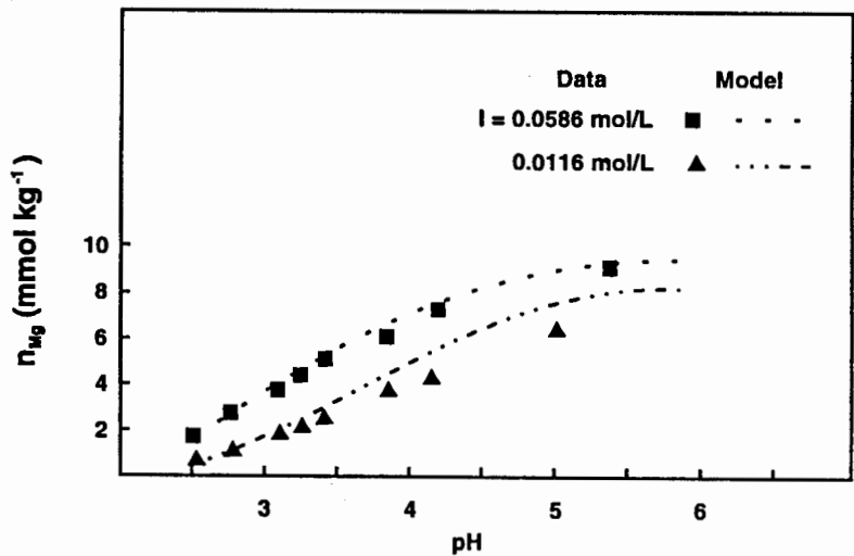
Fig. 10-11. Fit of the triple layer model to magnesium adsorption on a Brazilian oxisol (from Charlet, 1986).
