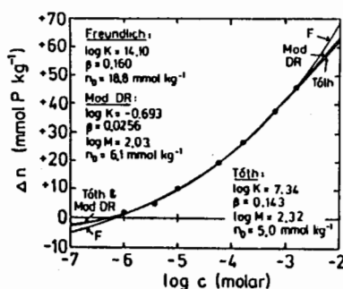
Fig. 10-3. Fit of various adsorption isotherm equations to phosphate adsorption on a Scottish soil (from Kinniburgh, 1986).
