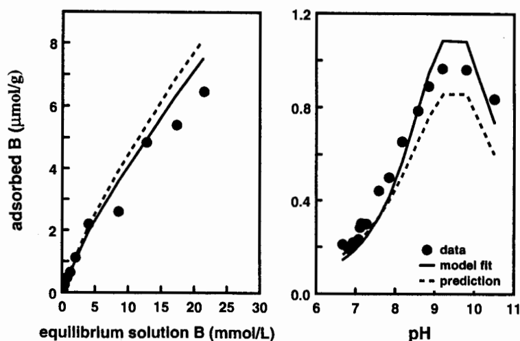
Fig. 10-A2. Constant capacitance model predictions of boron adsorption on a California soil as a function of solution B concentration and solution pH.
