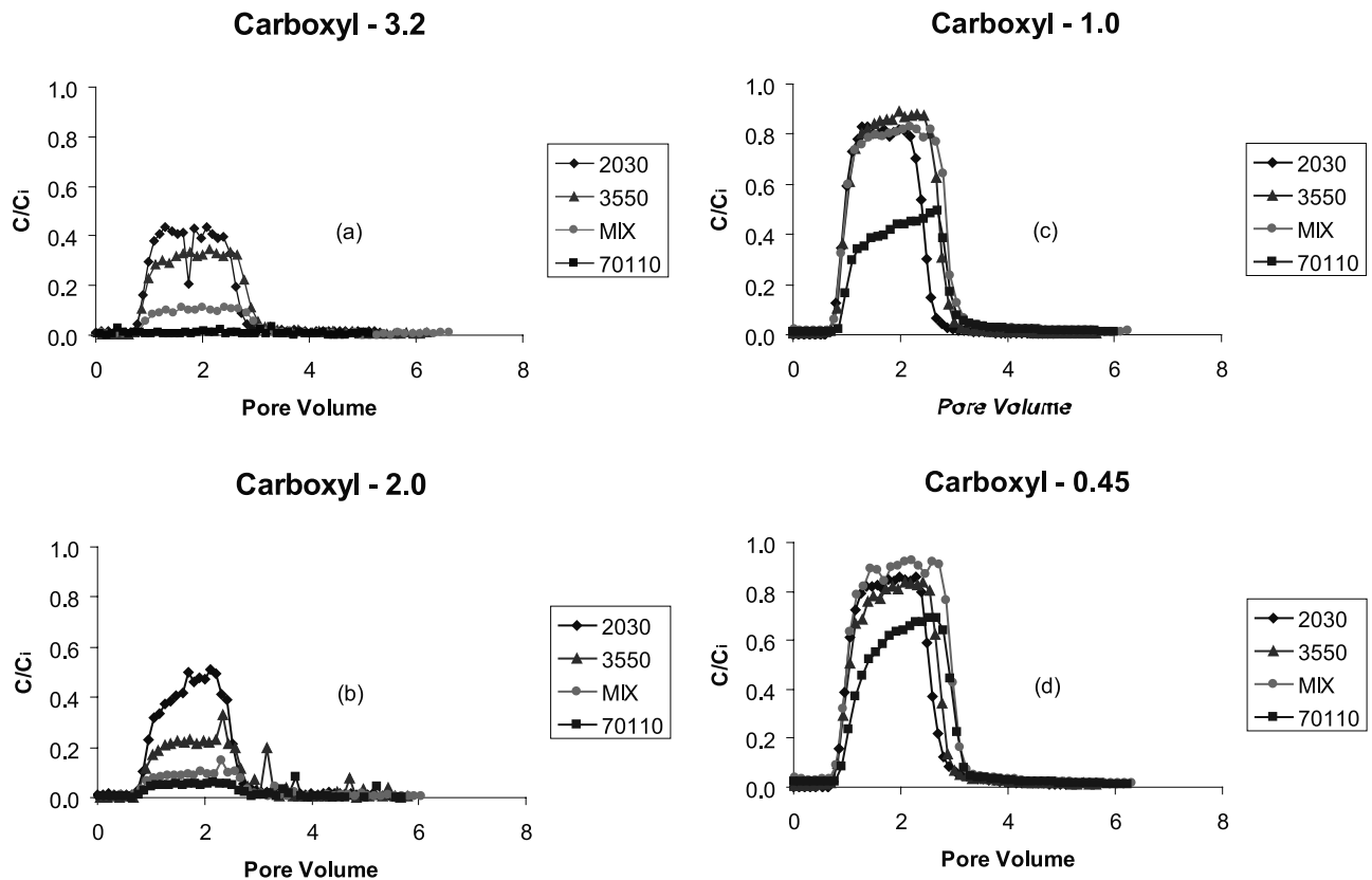
Figure 4. A plot of the relative colloid concentration in the effluent as a function of pore volume for the indicated colloid sizes (Figure 4a, 3.2 \mu\text{m} ; Figure 4b, 2.0 \mu\text{m} ; Figure 4c, 1.0 \mu\text{m} ; and Figure 4d, 0.45 \mu\text{m} ) and for the various soil types (2030, 3550, MIX, and 70110).
