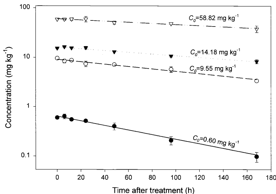
Fig. 3. Degradation of the (E)-1,3-dichloropropene isomer in Arlington sandy loam at different initial concentrations at 20°C. The points are mean of three measurements ( \pm standard errors) and the curves are first-order fits.
