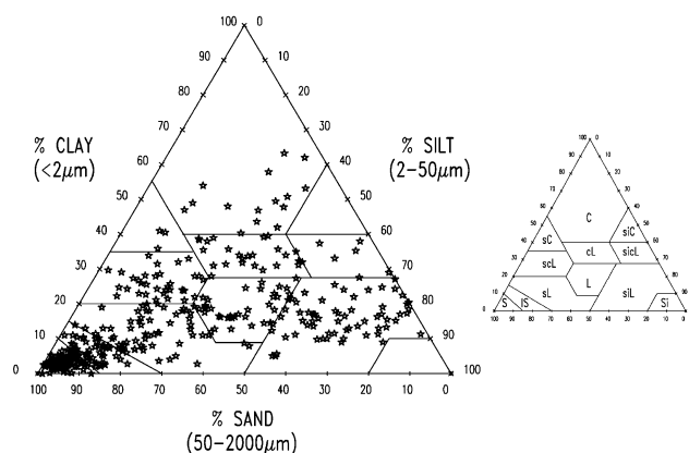
Fig. 2. Distribution of 431 soil codes in UNSODA V2.0 across the USDA-SCS soil textural triangle.
