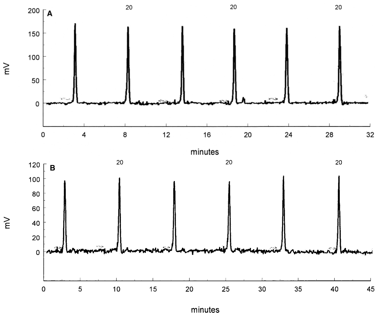
Fig. 2. Reproducibility of the IC-HGAAS method for multiple injections of a 20 µg L -1 standard: A) Se(IV); B) Se(VI).
