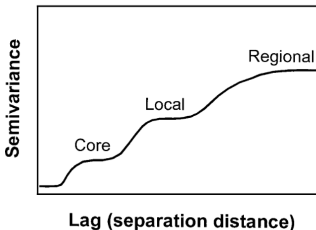
Fig. 2. Hypothetical variogram for scale-dependent hydraulic conductivity (redrawn from Gelhar, 1986).
