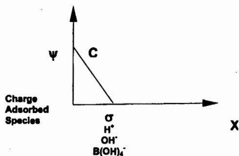
Figure 10. Placement of ions, capacitance, surface charge, \sigma , and surface potential, \psi for the constant capacitance model
