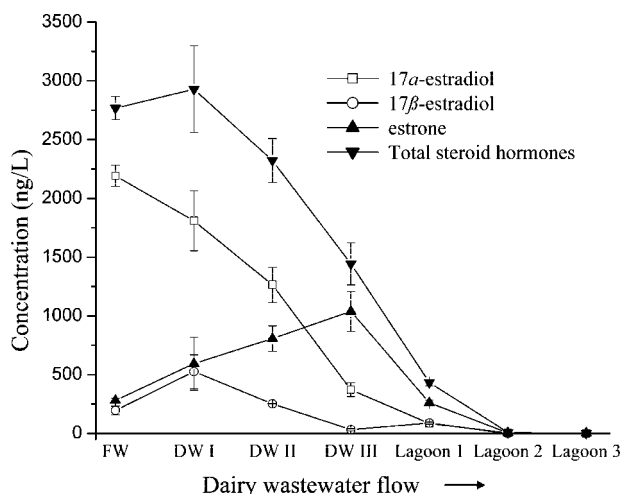
FIGURE 2. Concentration trends of steroid hormones along dairy wastewater flow. Abbreviations are as described in the text. Data shown are mean with standard deviation from six samples for each location that was sampled twice (November 2006 and March 2007).
