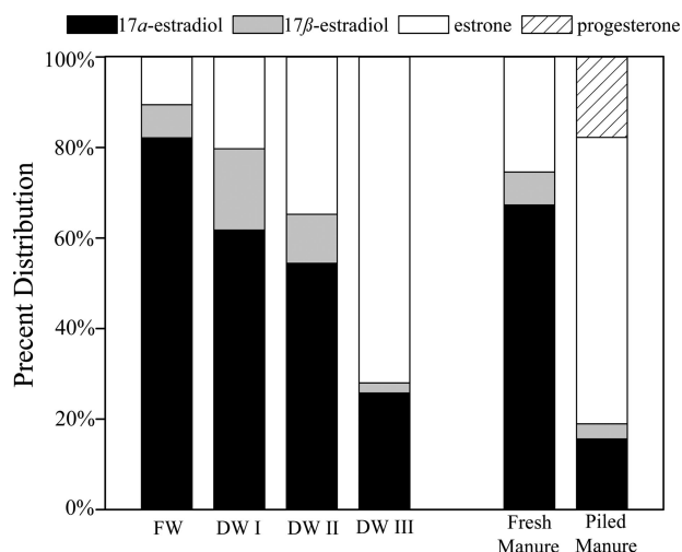
FIGURE 3. Percent distribution of each steroid hormone for total hormone equivalents. Abbreviations are as described in the text ( n = 6 for each type of sample).
