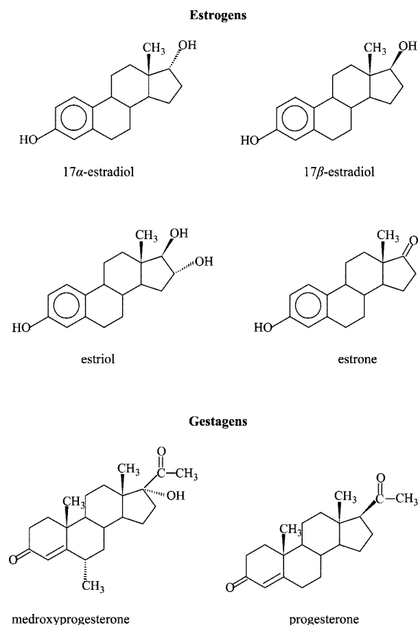
FIGURE 1. Structures of six steroid hormones of concern.
