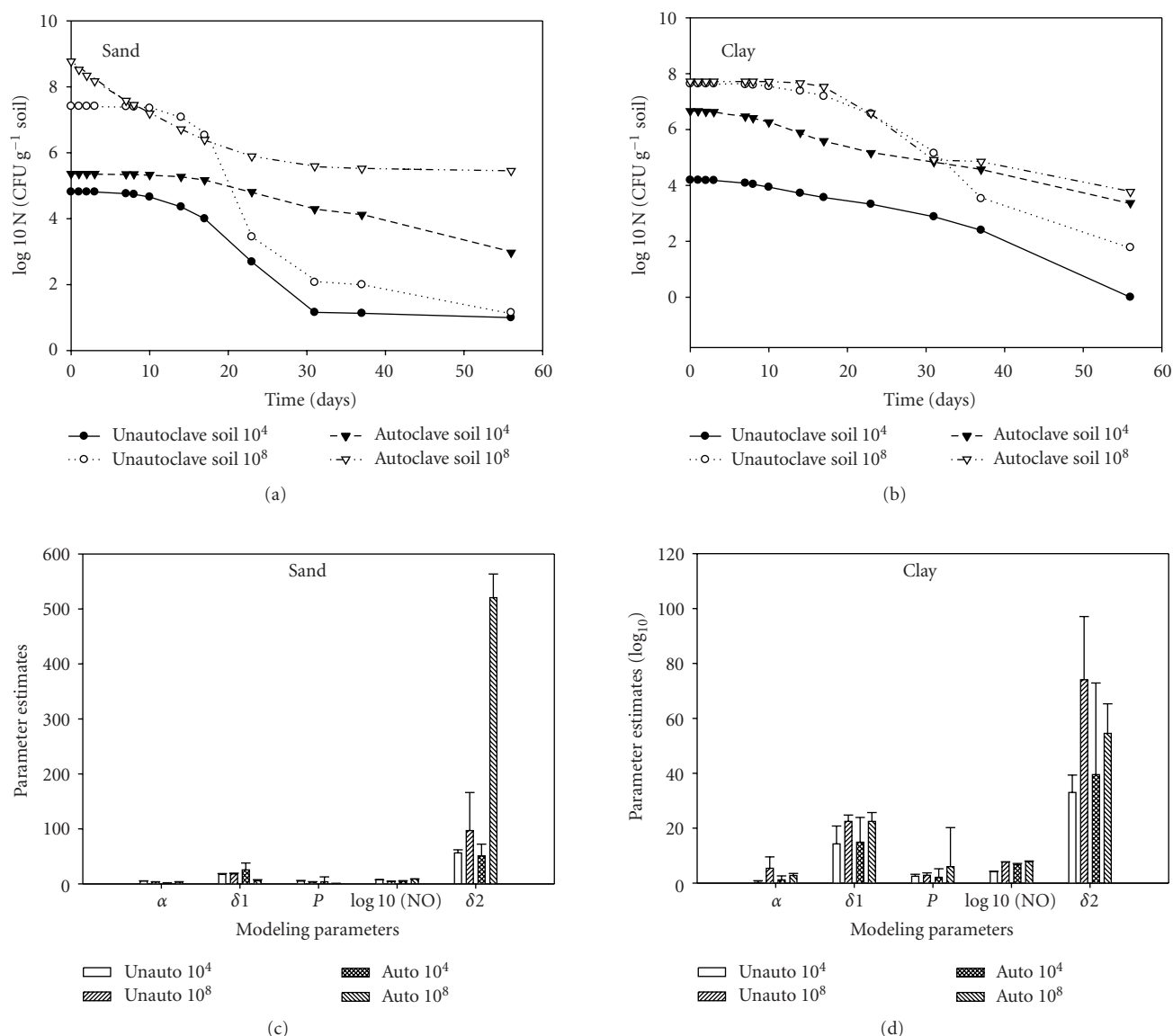
FIGURE 1: Survival of E. coli O157:H7 in autoclaved and unautoclaved (a) sand and (b) clay soils after 60 days incubation in a growth chamber at 20°C. E. coli O157: H7 was enumerated on TSA-ampicilin plates from soil with different concentrations of pathogen. Each point represents the average of triplicate sampling, and the bars at each point indicate survival coefficient obtained at each sampling point. All were log transformed as reported in the text. Double Weibull model parameters of E. coli O157:H7 in autoclave and nonautoclave sandy and clay soils (c, d)
