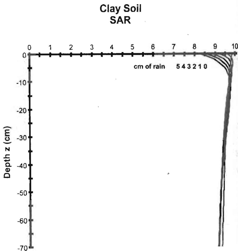
FIGURE 28-13. Relationship of SAR with depth and quantity of rain infiltrated into clay soil. The initial condition was SAR = 10 . Each curve represents addition of 1 cm of rain. From Suarez et al. (2006).
