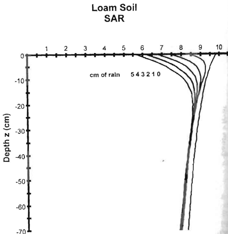
FIGURE 28-11. Predicted relationship of SAR with depth and quantity of rain infiltrated. The initial condition was EC = 1.0 \text{ dS/m} and SAR = 10 . Each curve represents addition of 1 cm of rain. From Suarez et al. (2006).
