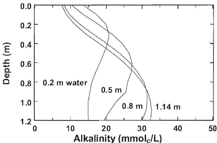
FIGURE 28-9. Model-predicted alkalinity concentrations ( \text{mmol/L} ) with depth after elevating the \text{CO}_2 to 5 kPa in the presence of calcite, and then leaching with 20, 50, 80, and 114 cm of water. From Suarez (2001).
