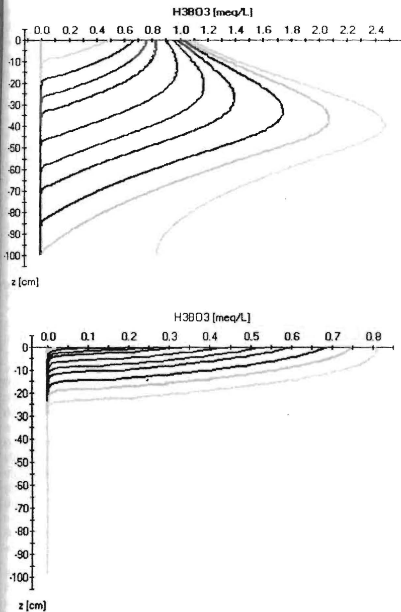
Figure 28-15. Change in boron concentration with depth and time (0, 10, 20, 30, 40, 50, 60, 70, 80, 90, and 100 days) for leaching fraction of 0.1 and soil surface area of (a) 100 \text{ m}^2 \text{ g}^{-1} , and (b) 1,000 \text{ m}^2 \text{ g}^{-1} . From Goldberg and Suarez (2006).
