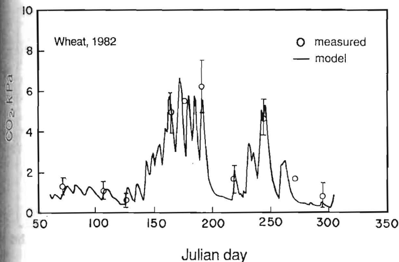
FIGURE 28-2. Measured (Buyanovsky and Wagner 1983) and calculated \text{CO}_2 concentrations at a depth of 0.20 m for a Missouri wheat experiment, 1982. Vertical bars show standard deviations. From Suarez and Šimůnek (1993).
