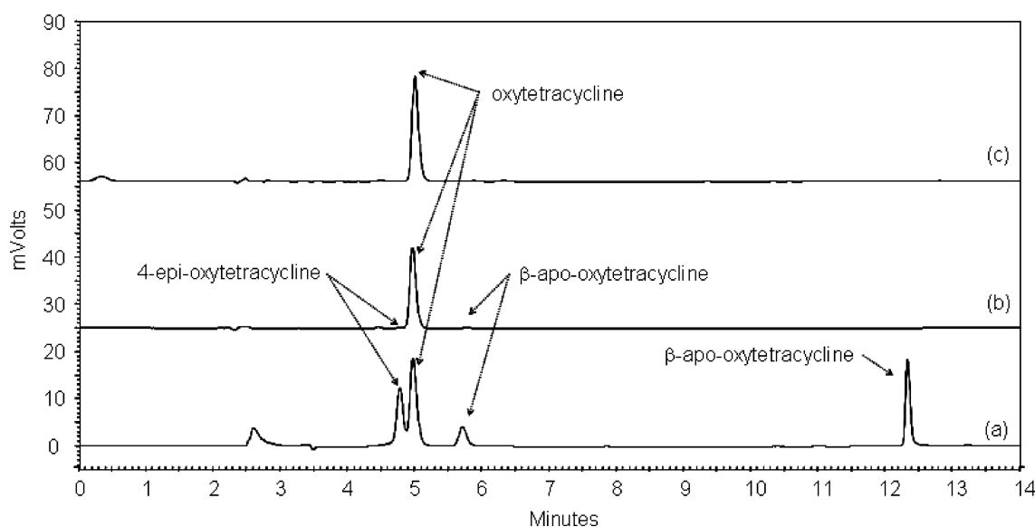
Fig. 1. Typical high performance liquid chromatography (HPLC) spectra of (a) standards, (b) oxytetracycline degradation solution at pH 9.06 without Ca 2+ after 10 days, and (c) oxytetracycline degradation solution at pH 9.78 with 1 mM Ca 2+ after 10 days.
