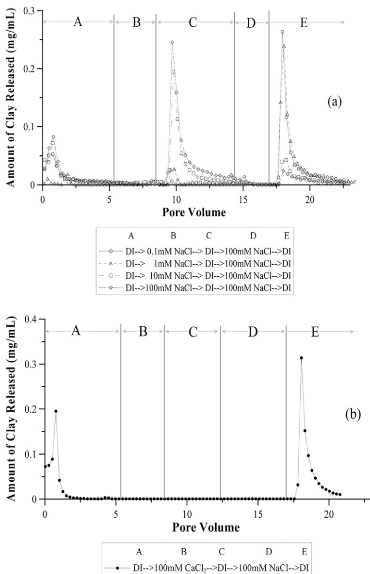
Fig. 4. The effluent concentration of clay released from 360- \mu m Ottawa sands as a function of pore volumes when the solution pH = 5.8. The solution chemistry sequence for the first column consisted of the following steps: (A) deionized (DI) water; (B) 0.1 mM NaCl; (C) DI water; (D) 100 mM NaCl; and (E) DI water. This same solution chemistry cycle was repeated for columns 2, 3, 4, and 5 but with 1 mM NaCl, 10 mM NaCl, 100 mM NaCl, and 100 mM CaCl 2 added during Step B, respectively. The duration of each aqueous solution pulse is given in Table 1, and the Darcy velocity was 0.27 cm min -1 .
