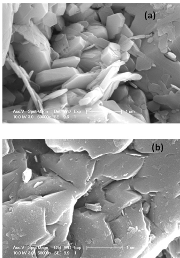
Fig. 5. Scanning electron microscope images of 360- \mu\text{m} Ottawa sand (a) before and (b) after using the cation exchange and ionic strength reduction cleaning protocol discussed in the text.
