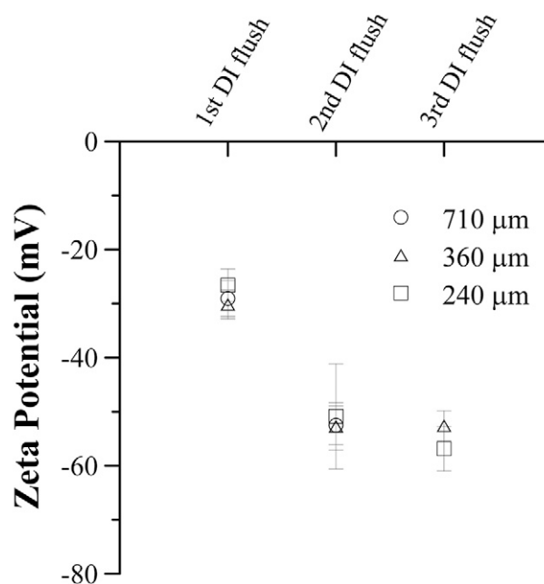
Fig. 2. Measured values of zeta potential for clay released during Steps A, D, and G shown in Fig. 1. Mean and standard deviation values of the clay zeta potentials are presented. DI, deionized water.
