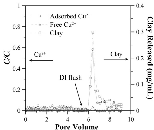
Fig. 6. Effluent concentrations ( C ) of clay and normalized concentration ( C/C_i ) of free \text{Cu}^{2+} in solution and \text{Cu}^{2+} adsorbed to clay as a function of pore volumes flushed through 360- \mu\text{m} Ottawa sand. The following solution chemistry sequence was followed: (A) 100 mM \text{NaCl} +2.5 \text{mg L}^{-1} \text{Cu}^{2+} ; (B) 100 mM \text{NaCl} ; and (C) deionized (DI) water. The duration of each aqueous solution pulse is provided in Table 1, and the Darcy velocity was 0.27 \text{cm min}^{-1} . The value of the influent \text{Cu}^{2+} concentration ( C_i ) was 2.5 \text{mg L}^{-1} .
