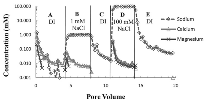
Fig. 3. A semi-log plot of the effluent concentrations of Na + , Ca 2+ , and Mg 2+ (mM) as a function of solution pore volumes that were passed through a column packed with 360- \mu m Ottawa sand. The influent solution chemistry sequence (pH = 5.8) consisted of the following steps: (A) deionized (DI) water; (B) 1 mM NaCl; (C) DI water; (D) 100 mM NaCl; and (E) DI water. The duration of each aqueous solution pulse is given in Table 1, and the Darcy velocity was 0.27 cm min -1 .
