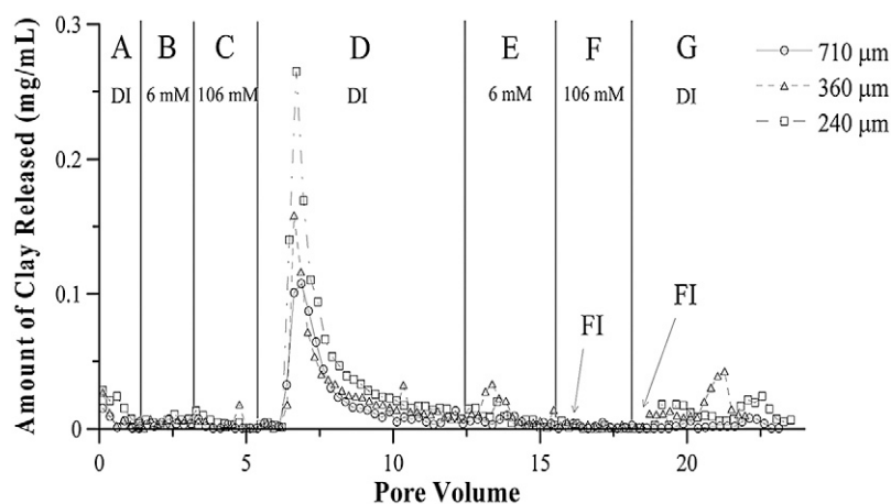
Fig. 1. The effluent concentration of clay released from 710-, 360-, and 240- \mu\text{m} Ottawa sands as a function of pore volume. The solution chemistry sequence consisted of the following steps: (A) deionized (DI) water at pH = 5.8; (B) 1 mM NaCl in pH = 10 solution (total ionic strength [IS] = 6 mM); and (C) 100 mM NaCl in pH = 10 solution (total IS = 106 mM). This same solution chemistry cycle was repeated during Steps D, E, and F followed by an additional pulse of DI water at pH = 5.8 during Step G. The duration of each aqueous solution pulse is given in Table 1, and the steady-state Darcy velocity was maintained at 0.27 \text{cm min}^{-1} . Periods of flow interruption are denoted with FI.
