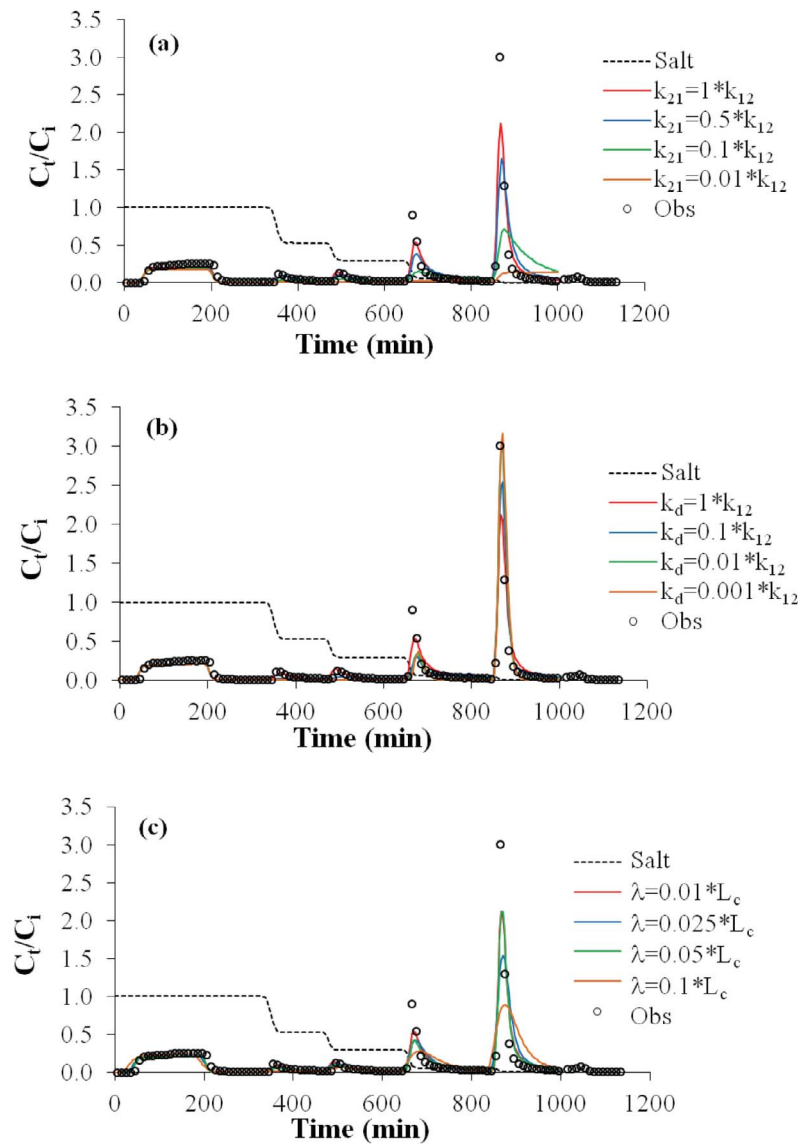
Figure 4. Observed and simulated transport and release behavior for 1.1 \mu\text{m} CML colloids when phases 1 and 2 were conducted at IS = 106 mM and phase 3 consisted of step decreases in IS equal to 56, 31, 6, and 0 mM. The values of (a) k_{21} , (b) k_d , and (c) \lambda are systematically varied. Other model parameters are given in Table 1.
