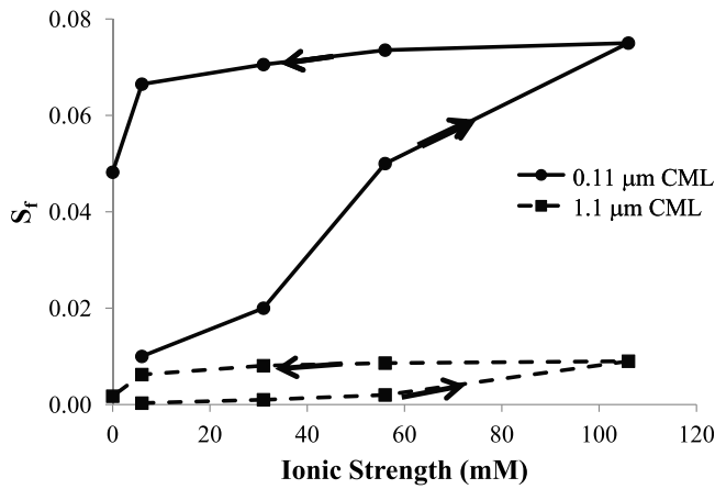
Figure 2. Hysteretic values of S_f for 0.11 and 1.1 \mu\text{m} CML colloids when phases 1 and 2 (arrow to the right) were conducted at \text{IS} = 106 \text{ mM} and phase 3 (arrow to the left) consisted of step decreases in IS equal to 56, 31, 6, and 0 mM. Experimental values of S_f were obtained by optimization of the simulated and measured breakthrough curves during phases 1 and 2, whereas equation (17) was used to predict S_f during phase 3.
