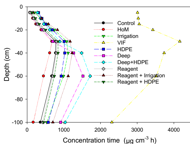
Fig. 3. Predicted Mel concentration-time values along soil depths for the Control, irrigation, HOM, VIF, HDPE, Deep, Deep + HDPE, Reagent, Reagent + Irrigation, and Reagent + HDPE treatments.
